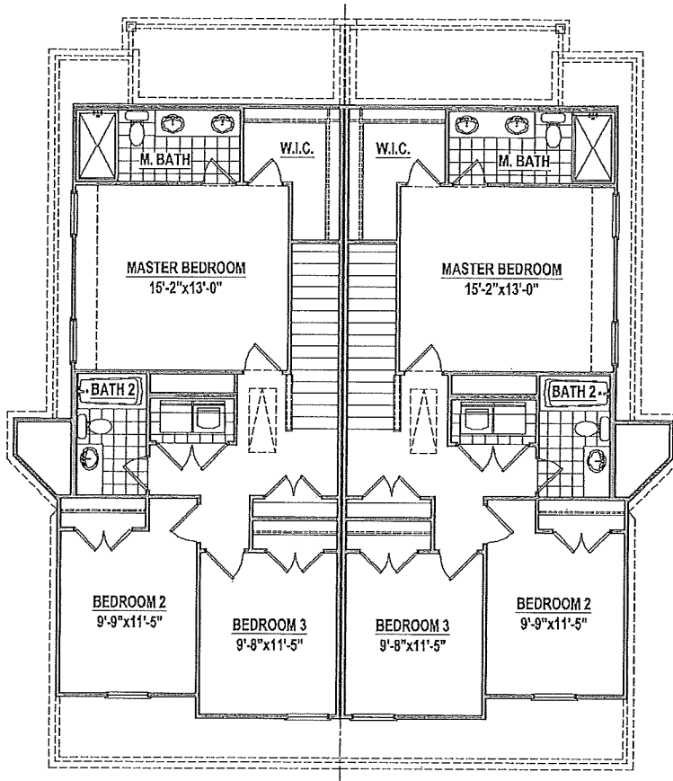
UNIT A SECOND FLOOR
